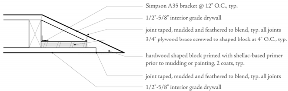
12 Sill/Jamb Detail at Aperture Opening Scale: 1-1/2" = 1'-0"
